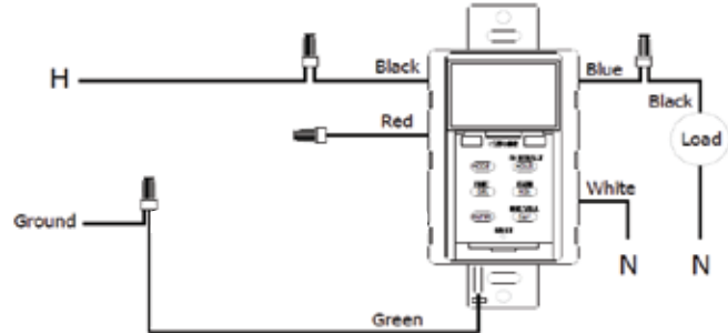
Wiring Diagram: Installation SS721Z
