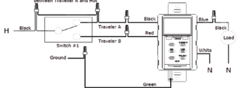
Wiring Diagram: Three-Way Installation S721Z
