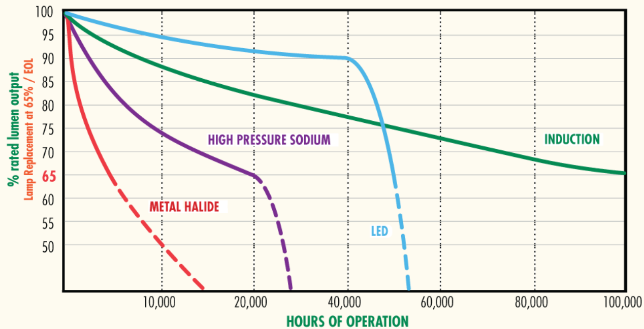
ESTIMATED LUMEN MAINTENANCE
